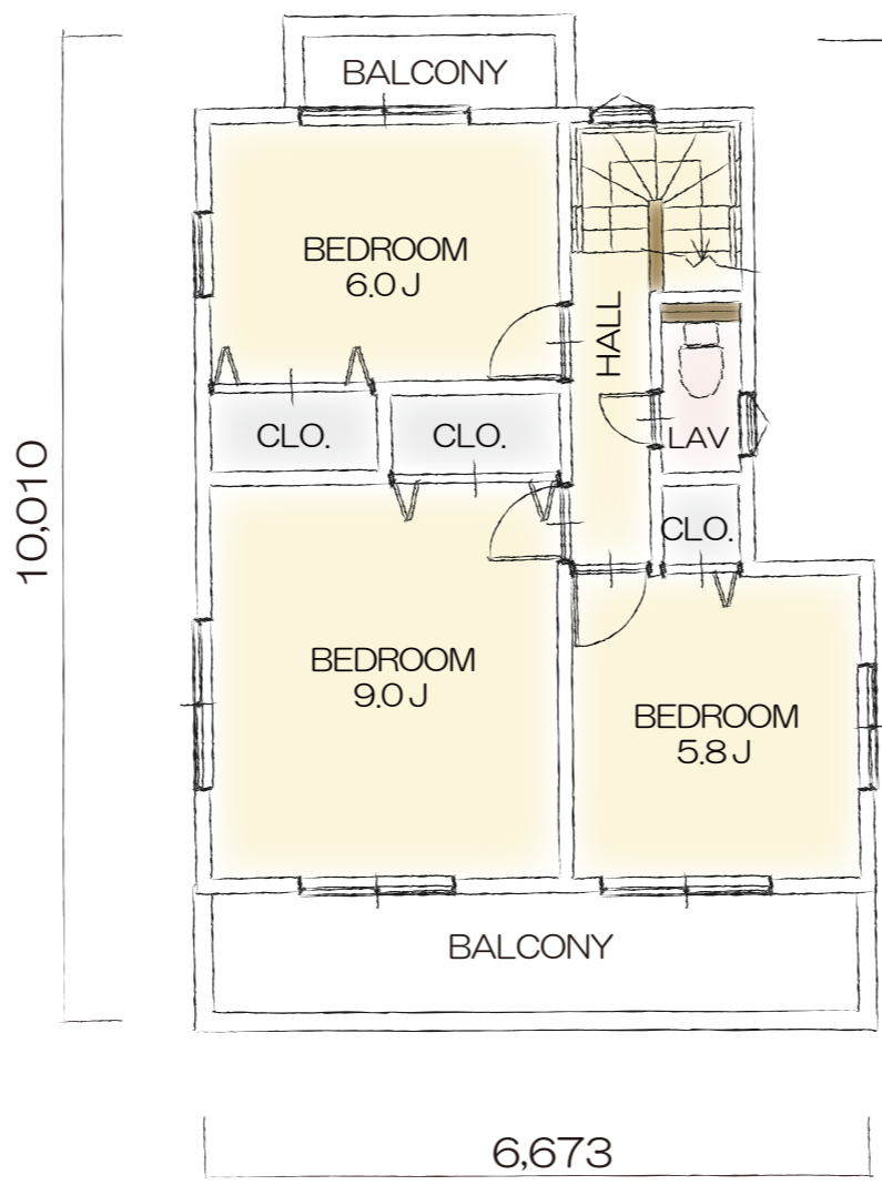
2F PLAN
